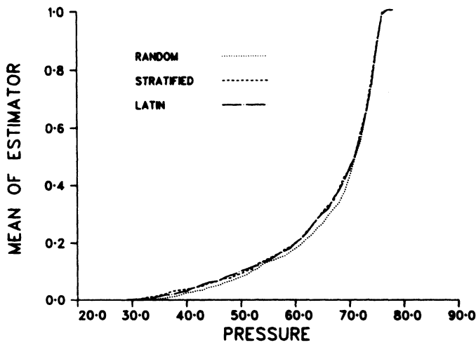
Figure 5. Estimating the CDF: The Sample Mean of G_R(y, t) , G_S(y, t) , and G_L(y, t) at t = 1.4 .
